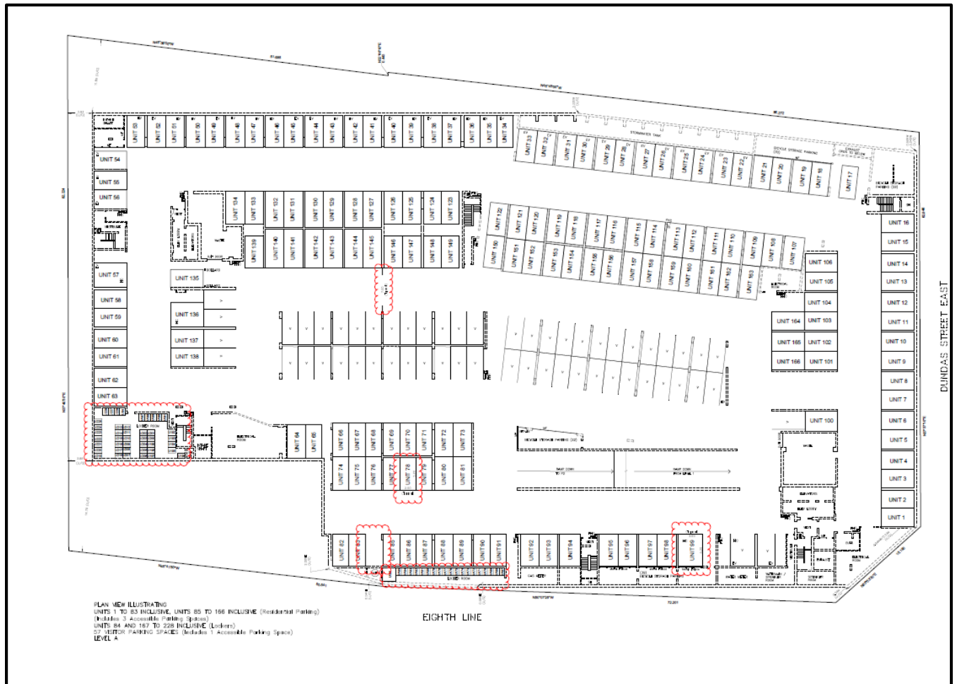
Figure 9 – Draft Plan of Condominium Parking Level A
