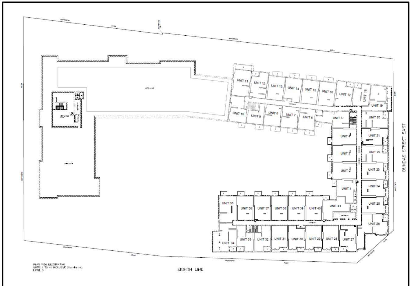
Figure 5 – Draft Plan of Condominium Level 5
