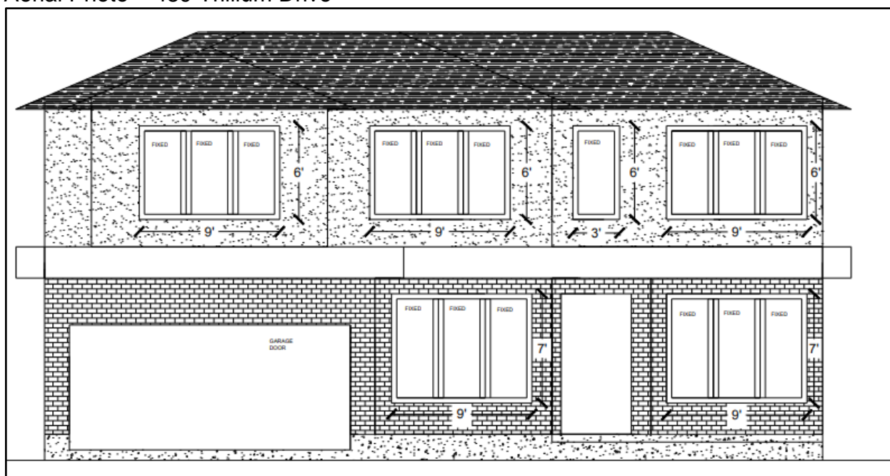
Front Elevation – 489 Trillium Drive
