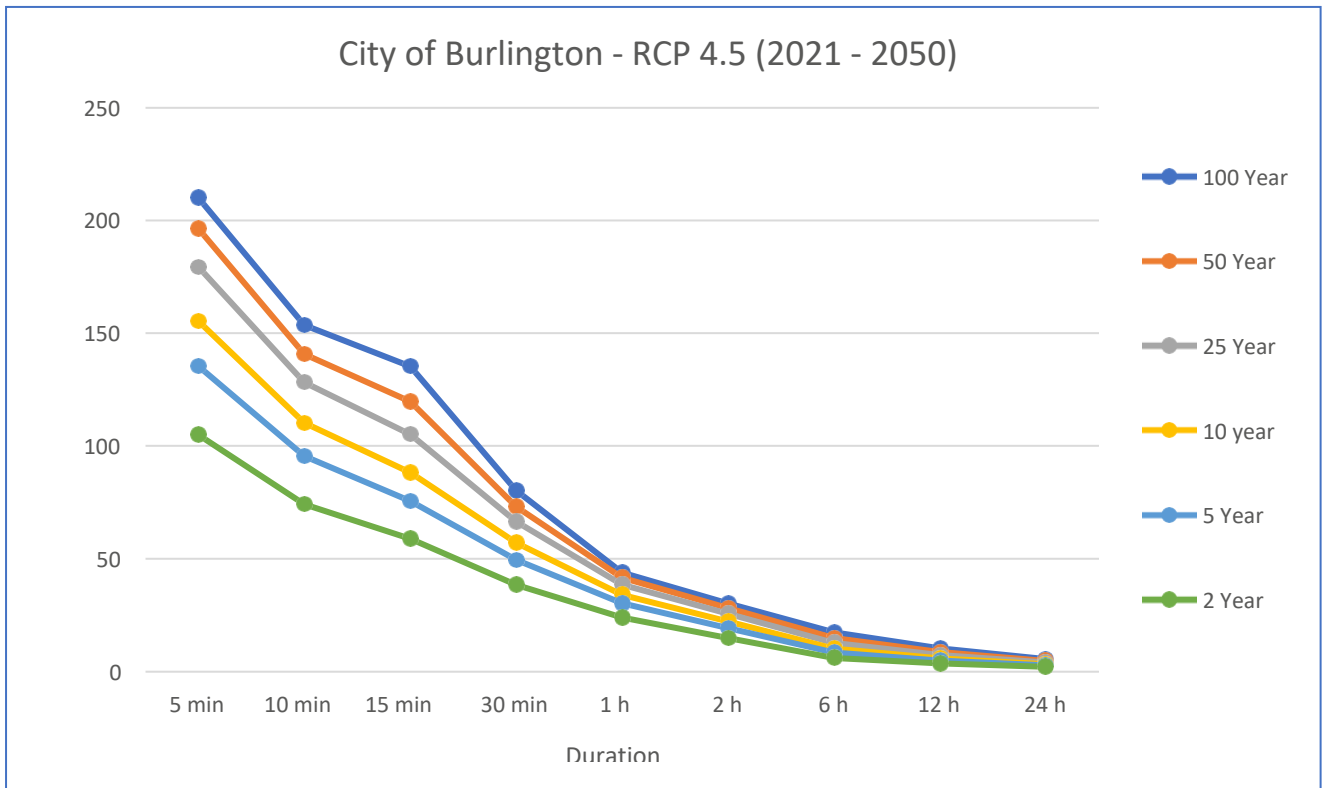
Figure B1: Rainfall Intensity Rates (mm/h) for City of Burlington – RCP4.5 (2021-2050)
