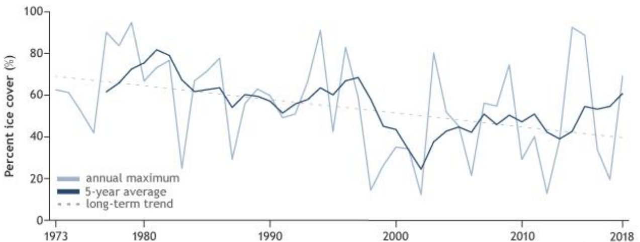
Figure 21: Time Series of Yearly Maximum Ice Cover in the Great Lakes (1973-2018)
