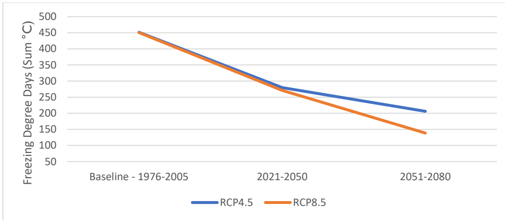
Figure 9: Freezing Degree Days for Burlington Region - RCP4.5 and 8.5
