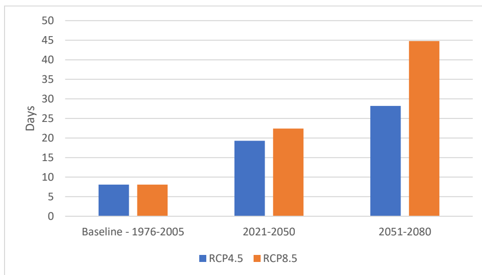
Figure 5: Annual Tropical Nights for Burlington Region - RCP4.5 and 8.5
