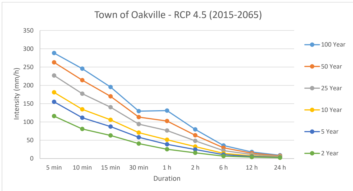
Figure C1: Rainfall Intensity Rates for Town of Oakville
