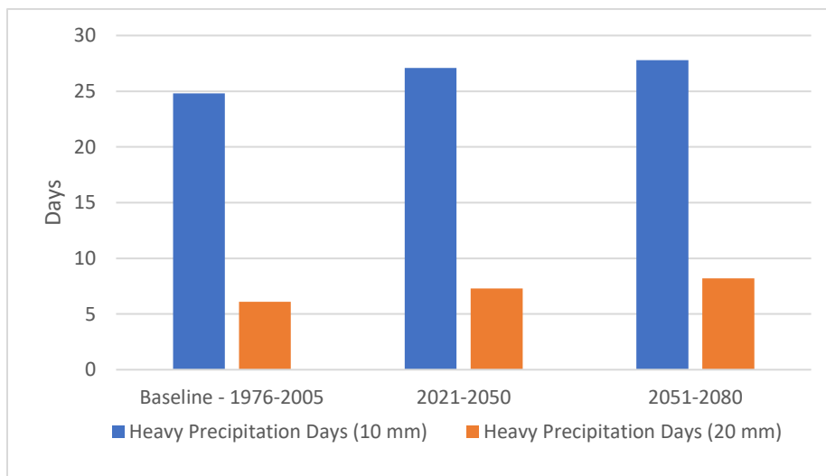
Figure 12: Heavy Precipitation Days for Burlington Region - RCP8.5
