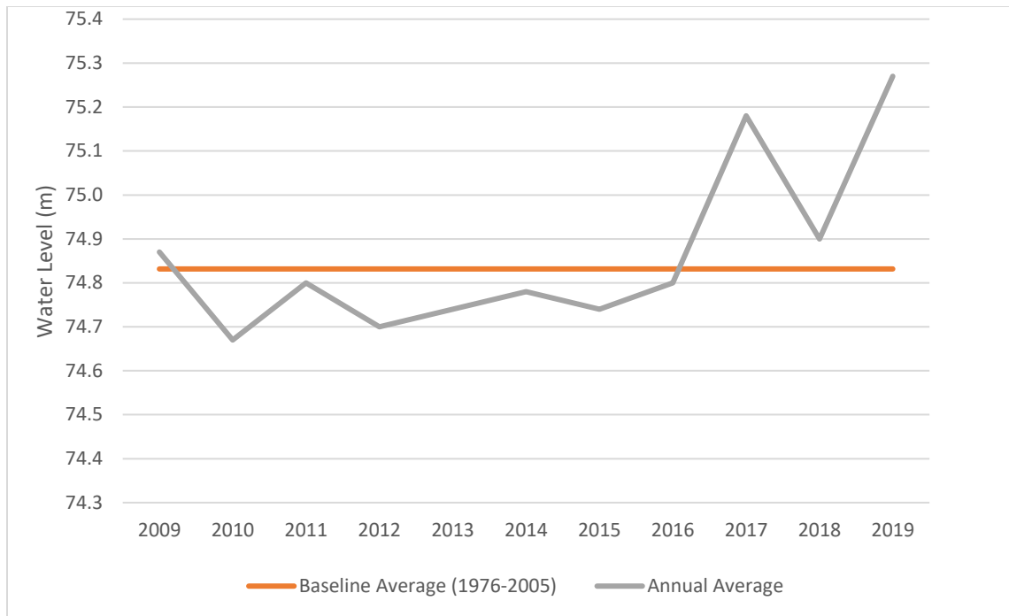
Figure 18: Annual Water Levels (2009-2019) Compared to the Baseline
