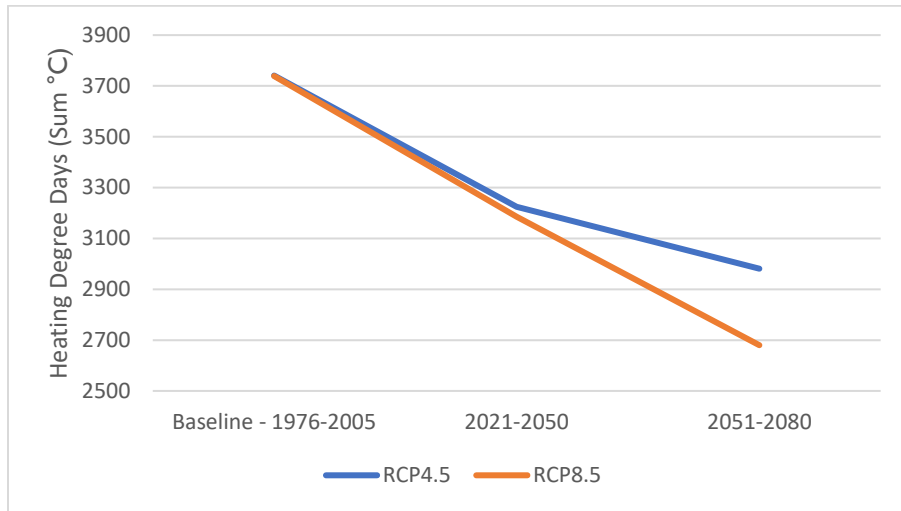
Figure 8: Heating Degree Days for Burlington Region - RCP4.5 and 8.5
