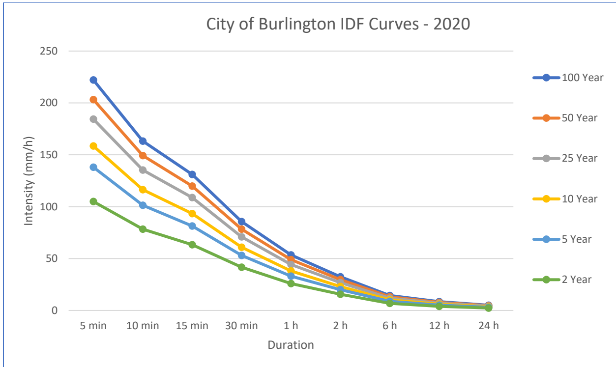
Figure 16: City of Burlington 2020 IDF curve
