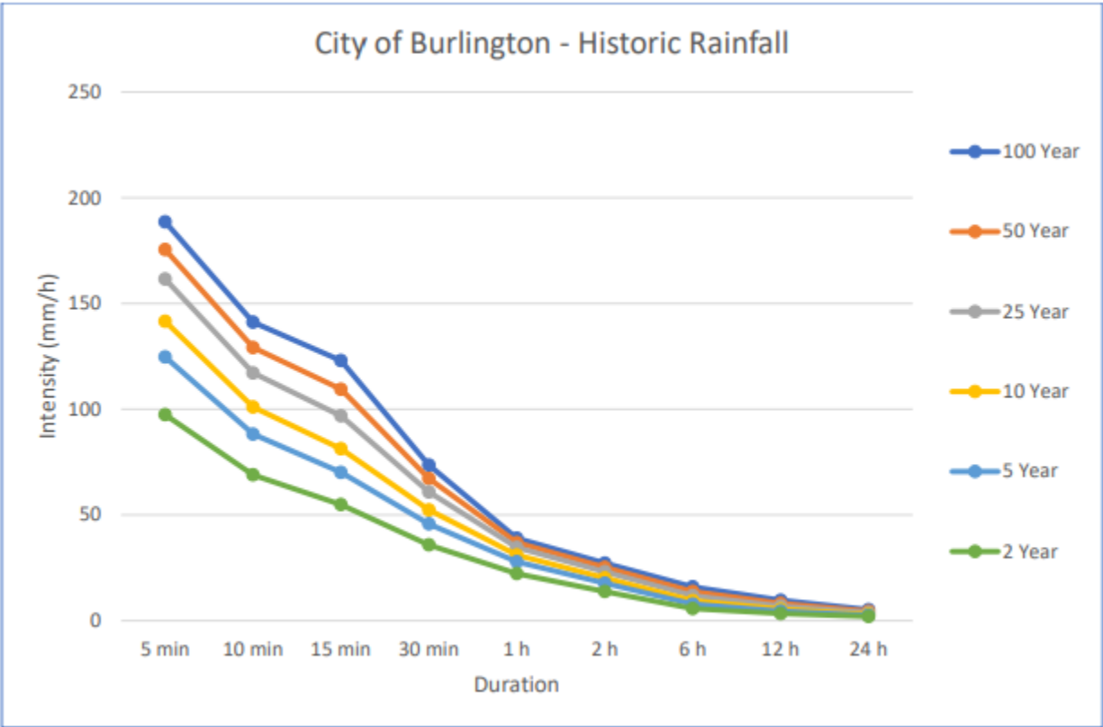
Figure 15: Historical IDF Curve for the City of Burlington (1962-2016)
