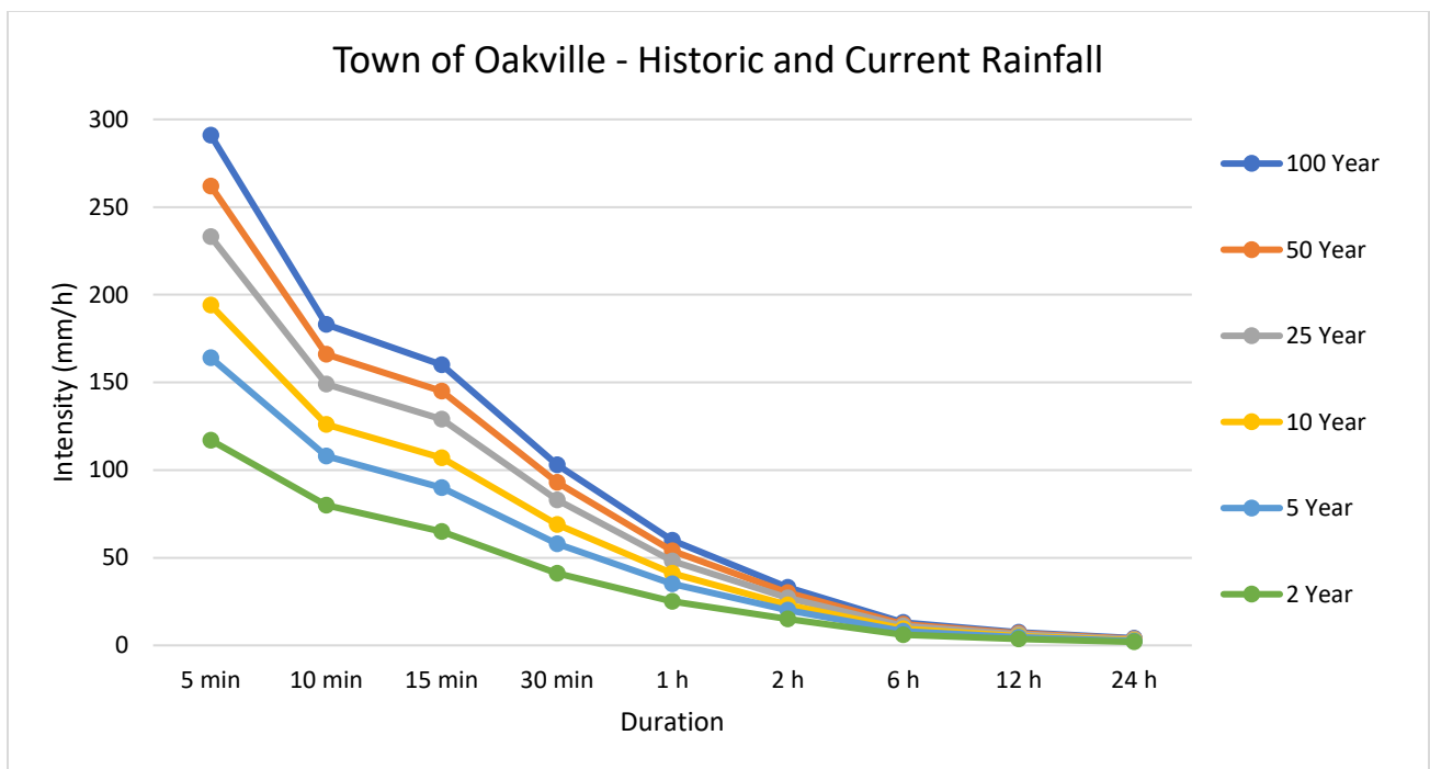
Figure 17: Historic and Current IDF Curve for the Town of Oakville (1946-2007)
