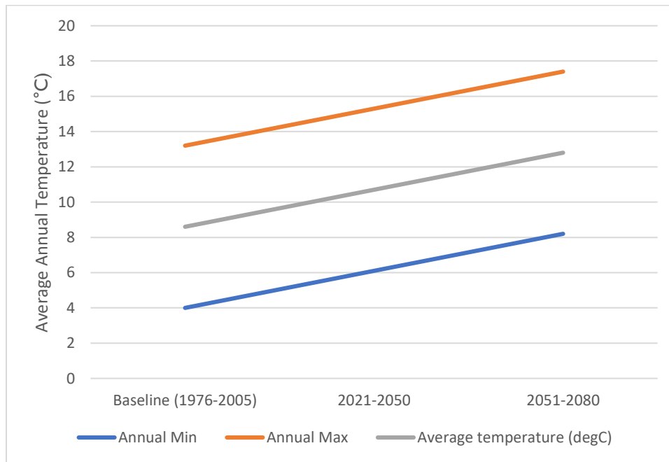
Figure 3: Annual Temperature for Burlington Region - RCP8.5
