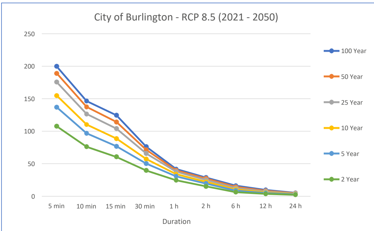
Figure B3: Rainfall Intensity Rates (mm/h) for City of Burlington – RCP8.5 (2051-2080)
