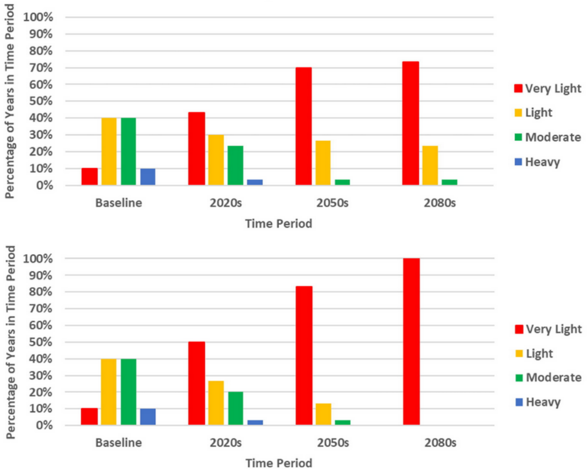
Figure 23: Projected Ice Conditions for Lake Ontario (2011-2100), based on RCP4.5 (top) and RCP8.5 (bottom), including the Baseline Time-Period for Context
