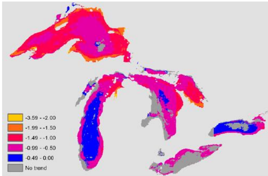
Figure 22: Seasonal Ice Cover Duration (days/year) (1973-2013)
