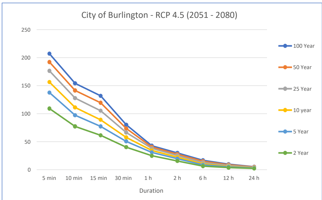
Figure B2: Rainfall Intensity Rates (mm/h) for City of Burlington – RCP4.5 (2051-2080)
