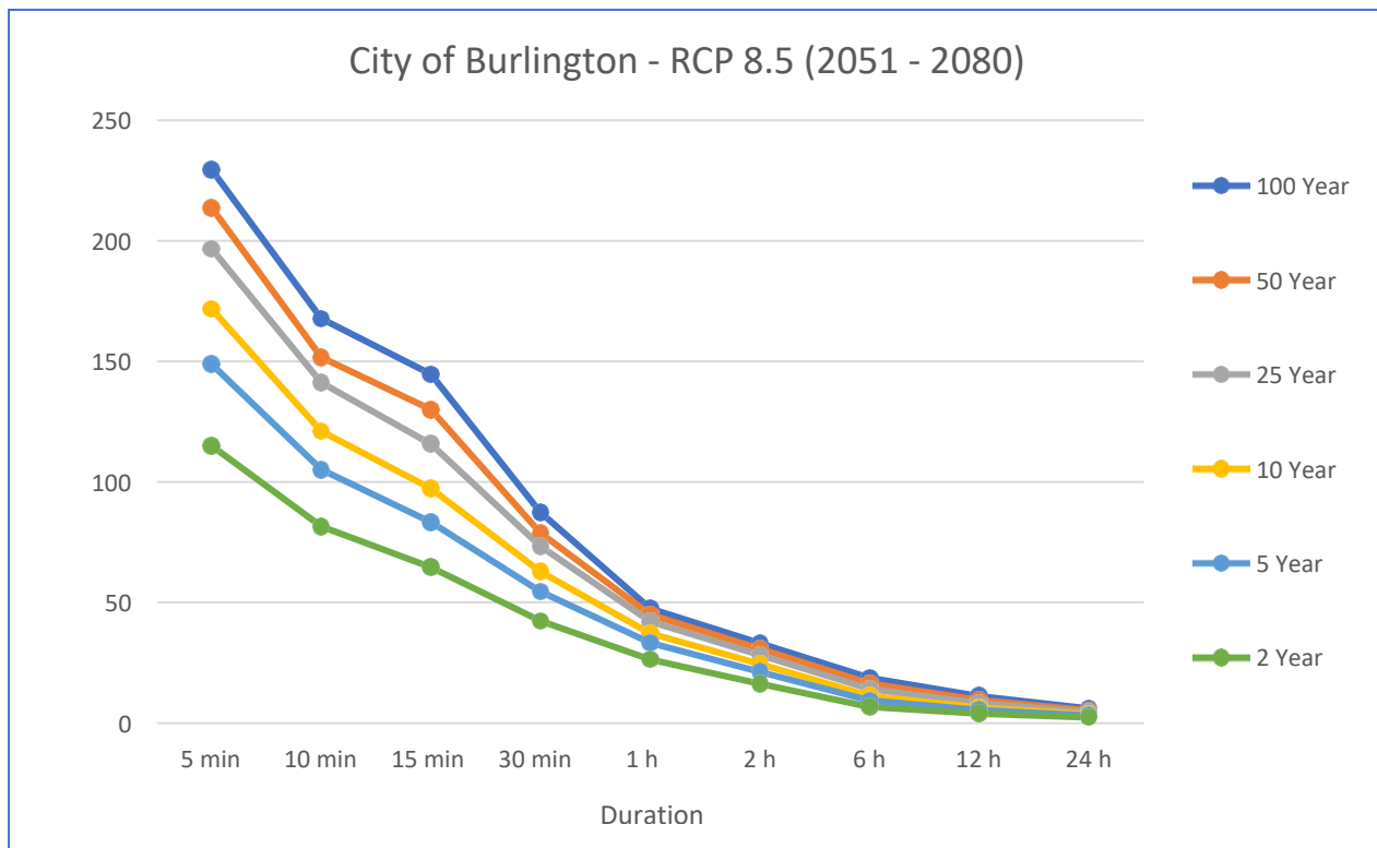
Figure B4: Rainfall Intensity Rates (mm/h) for City of Burlington – RCP8.5 (2051-2080)
