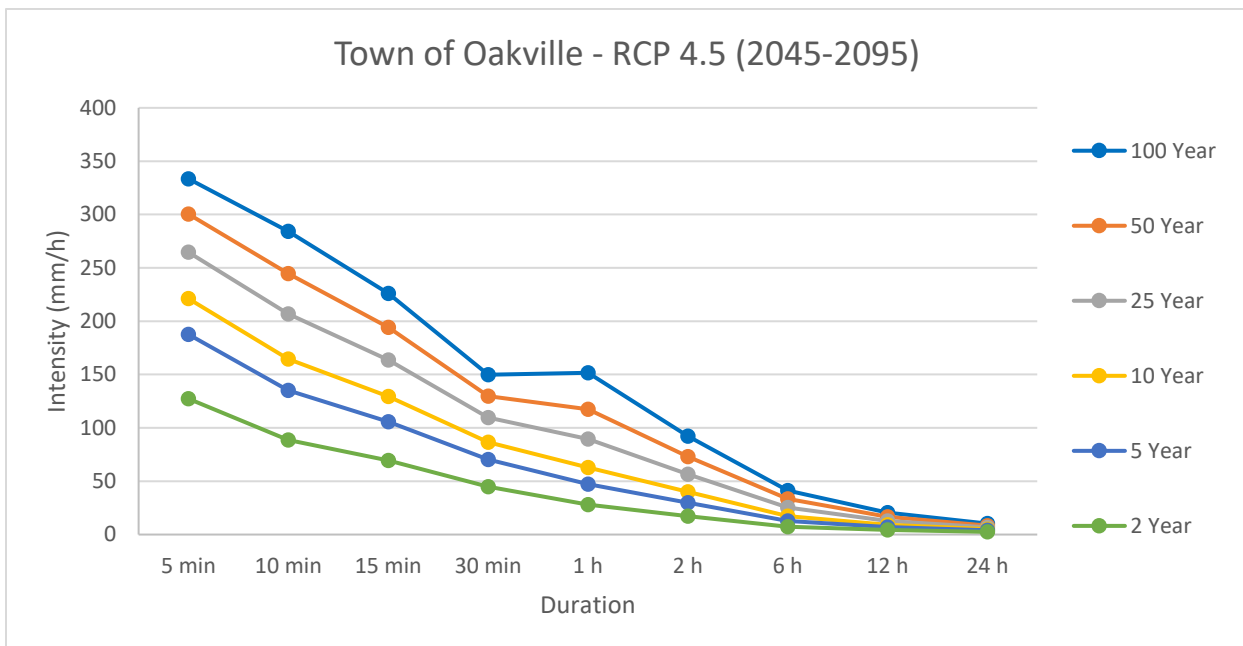
Figure C2: Rainfall Intensity Rates for Town of Oakville
