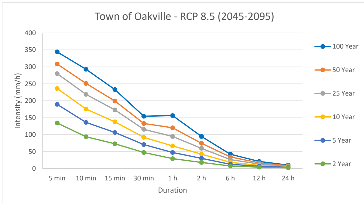
Figure C4: Rainfall Intensity Rates for Town of Oakville
